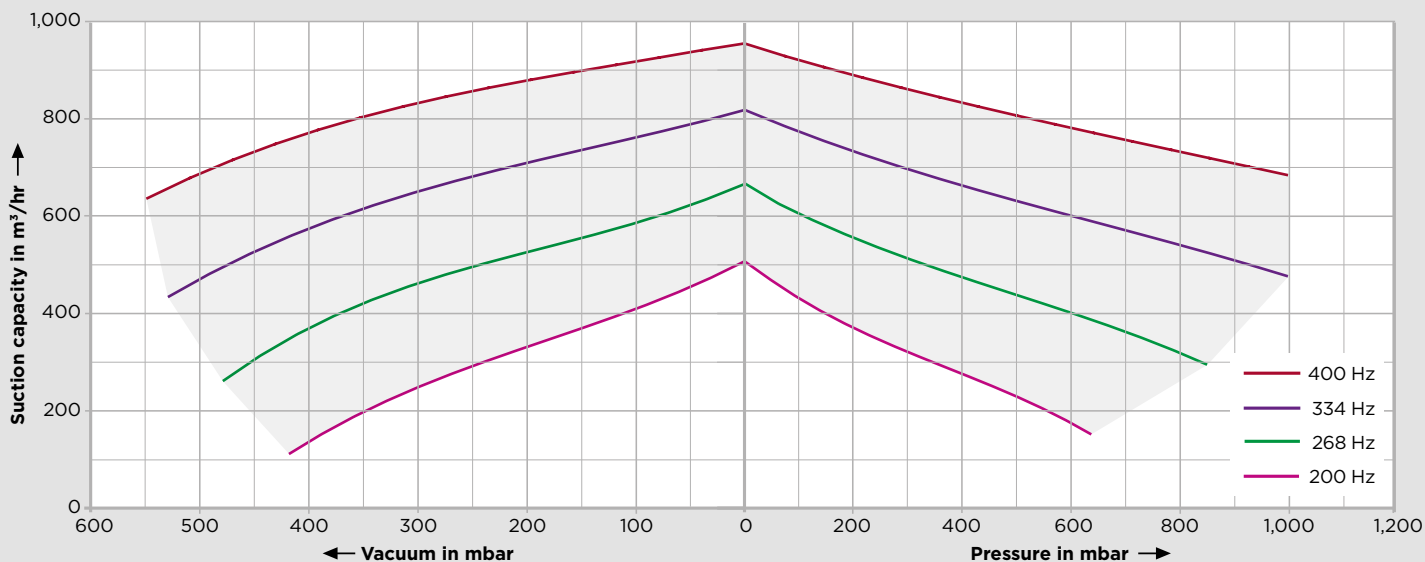
G-BH8 with silencer
